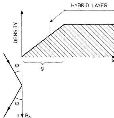
Fig. 1. The co-ordinate system.
