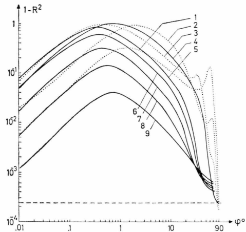
Fig. 10. Transmission coefficient vs \varphi for an incident TM wave for nine values of \omega/\omega_{ci} given in Table 2 using the parameters of Table 1.
