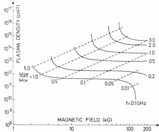
Fig. 19. The curves showing \omega_{pe}/\omega_{ce} as well as the lower-hybrid frequency f as functions of plasma density and magnetic field for deuterium. Region of accessibility corresponds to \omega_{pe}/\omega_{ce} \lesssim 0.4 .
