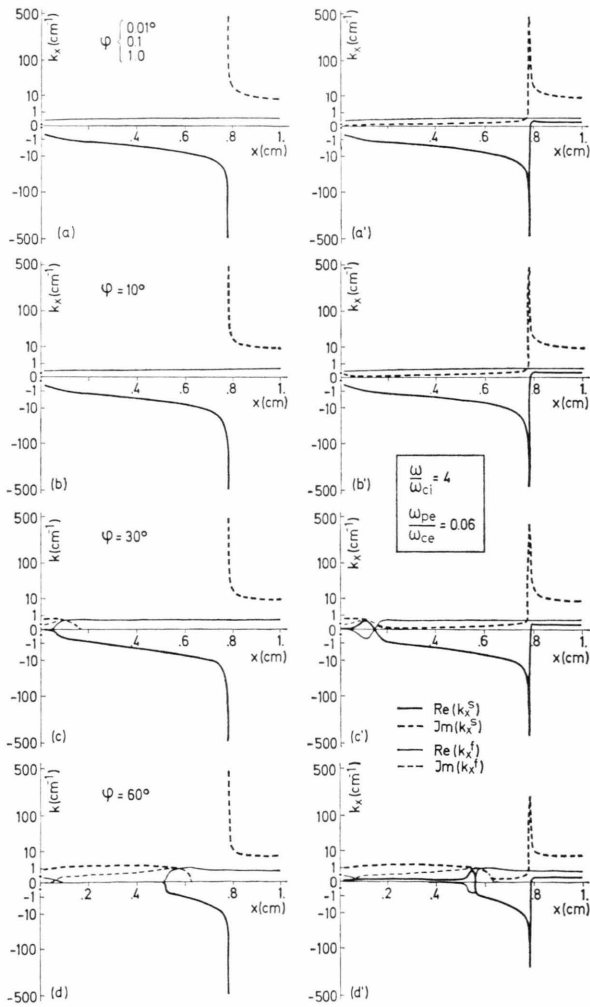
Fig. 16. The propagation constant k_x vs x for \omega/\omega_{ci}=4 for both the slow and the fast waves for four values of \varphi . The unprimed and the primed pairs are for T=\infty ( \nu_{ei}=0 ) and T=3\times 10^4 °K, respectively.
