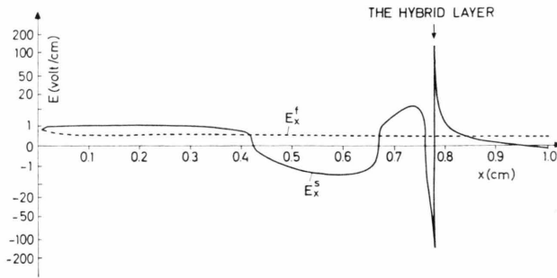
Fig. 2. The real part of the x -component of the electric field vs x for both the slow and the fast waves for the representative case of Section I. (The vertical scale is cubically compressed.)
