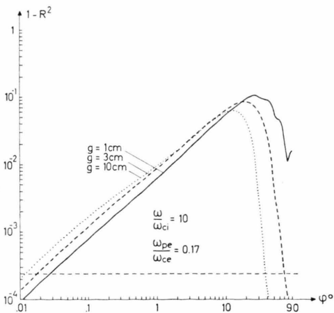
Fig. 15. Transmission coefficient vs \varphi for \omega/\omega_{ci}=10 ( \omega_{pe}/\omega_{ce}=0.17 ) for an incident TE wave for three different values of the profile width “ g ”. All other parameters are those of Table 1.
