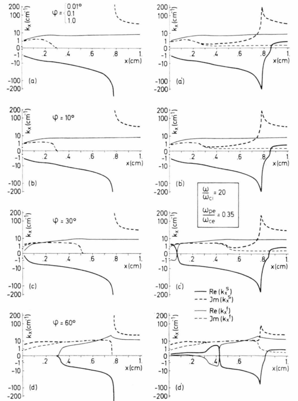
Fig. 18. The propagation constant k_x vs x for \omega/\omega_{ci}=20 for both the slow and the fast waves for four values of \varphi . The unprimed and the primed pairs are for T=\infty ( \nu_{ei}=0 ) and T=3 \times 10^4 °K, respectively.
