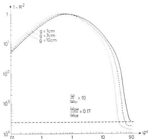
Fig. 13. Transmission coefficient vs \varphi for \omega/\omega_{ci} = 10 ( \omega_{pe}/\omega_{ce} = 0.17 ) for an incident TM wave for three different values of the profile width "g". All other parameters are those of Table 1.
