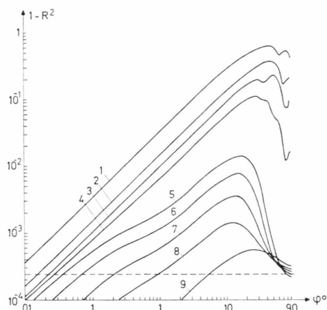
Fig. 11. Transmission coefficient vs \varphi for an incident TE wave for nine values of \omega/\omega_{ci} given in Table 2 using the parameters of Table 1.
