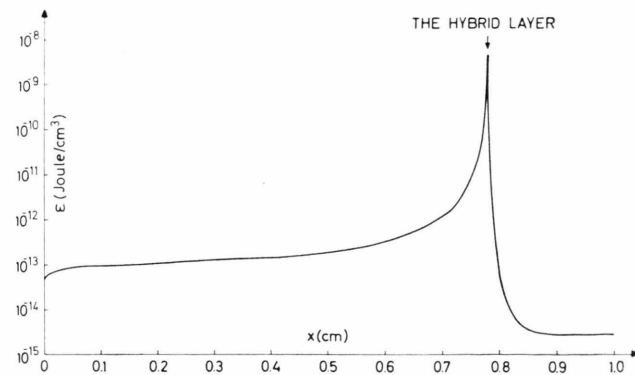
Fig. 4. Energy density \varepsilon = 1/4[\varepsilon_0 \mathbf{E}^* \cdot \partial(\omega \mathbf{K})/\partial \omega \cdot \mathbf{E} + \mu_0 \mathbf{H}^* \cdot \mathbf{H}] vs x .
