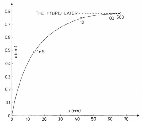
Fig. 7. Propagation of an energy pulse travelling with the group velocity of the slow wave from the plasma edge to the hybrid layer.
