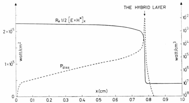
Fig. 3. Real part of the x -component of the Poynting vector [1/2(\mathbf{E} \times \mathbf{H}^*)]_x and the dissipation density -\nabla \cdot [1/2(\mathbf{E} \times \mathbf{H}^*)] vs. x .
