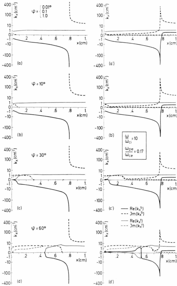
Fig. 17. The propagation constant k_x vs x for \omega/\omega_{ci}=10 for both the slow and the fast waves for four values of \varphi . The unprimed and the primed pairs are for T=\infty ( \nu_{ei}=0 ) and T=3 \times 10^4 °K, respectively.
