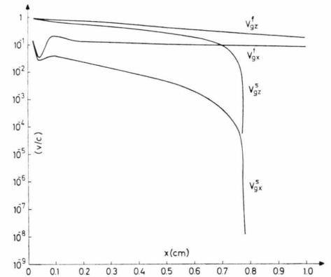
Fig. 6. The x and z -components v_{gx}/c and v_{gz}/c of the normalized group velocities for both the fast and the slow waves.
