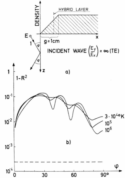
Fig. 9. Transmission coefficient as a function of \varphi and T for an incident TE wave using all other parameters as given in Table 1.
