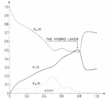
Fig. 5. Relative energy densities \varepsilon_i/\varepsilon , \varepsilon_e/\varepsilon and \varepsilon_v/\varepsilon in the ions, the electrons and the electromagnetic field, respectively.
