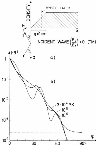
Fig. 8. Transmission coefficient ( 1-R^2 ) as a function of \varphi and T for an incident TM wave using all other parameters as given in Table 1.
